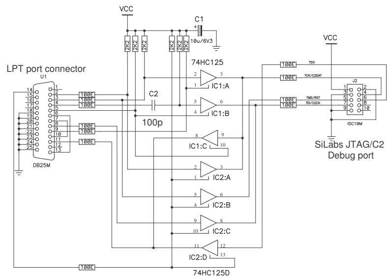
(14=VCC, 7=GND) FLASHBLASTER2 SCHEMATICS
